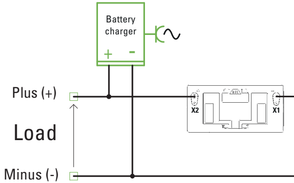
Figuur 17. Connecting a charger to the Li-ion battery
